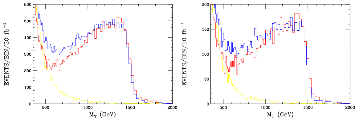
Figure 2: Same as in the previous figure but now on a linear scale with lower luminosities and smeared by the detector resolution. In the left (right) panel an integrated luminosity of 30(10) fb^{-1} has been assumed. Detector smearing has now been included assuming \delta M_T/M_T = 2\% .
