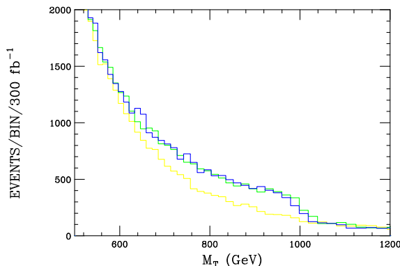
Figure 6: High luminosity plot of the transverse mass distribution assuming M_{W'} = 1 \text{ TeV} for the second W KK level in the UED model smeared by detector resolution as above. As usual the lower histogram is the SM background while the other two correspond to the signal cases with h_{W'} = -1(1) and are essentially indistinguishable.
