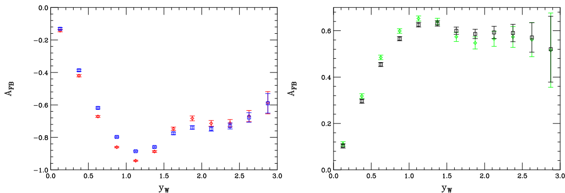
Figure 8: The value of A_{FB} as a function the center of mass rapidity, y_W , integrated over the transverse mass bin 400-1000 GeV assuming a mass of 1.5 TeV for the W'^+(W'^-) in the left (right) panel. An integrated luminosity of 300 \text{ fb}^{-1} has been assumed and the distribution has been folded around y_W = 0 . The upper(lower) set of data points in the left (lower) panel for small values of y_W corresponds to the choice of h_{W'} = -1 . Note that we have chosen signs to make the ranges of A_{FB} comparable in both cases.
