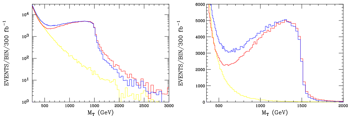
Figure 1: Transverse mass distribution for the production of a 1.5 TeV W' including interference effects at the LHC displayed on both log and linear scales assuming an integrated luminosity of 300 \text{ fb}^{-1} . The lowest histogram is the SM continuum background. The upper blue(middle red) histogram at M_T = 600 \text{ GeV} corresponds to the case of h_{W'} = -1(1) .
