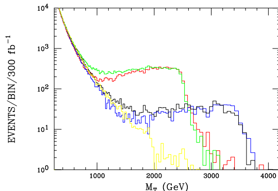
Figure 3: High luminosity plot of the transverse mass distribution assuming M_{W'} = 2.5(3.5) for the upper(lower) pair of histograms along with the SM continuum background. In the interference region near \simeq 0.5M_{W'} the upper(lower) member of the pair corresponds to the case of h_{W'} = -1(1) . Detector smearing has now been included assuming \delta M_T/M_T = 2\% .
