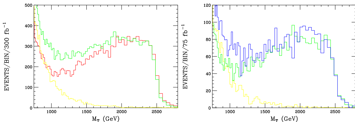
Figure 4: Transverse mass distribution assuming a mass of 2.5 TeV for the W' along with the SM continuum background; the upper(lower) panel corresponds to a luminosity of 300(75) fb^{-1} . In the interference region near \simeq 0.5M_{W'} the upper(lower) histogram corresponds to the case of h_{W'} = -1(1) .
