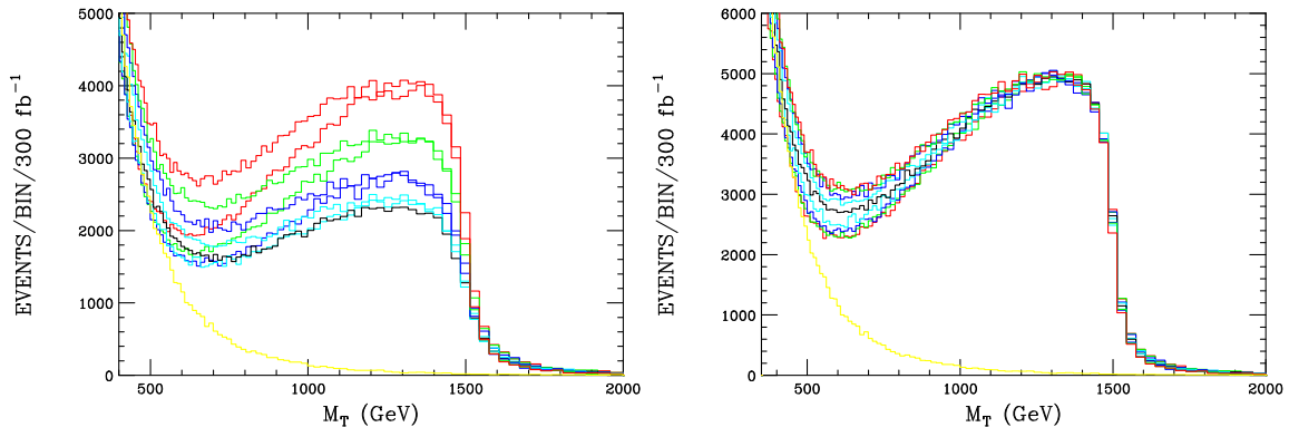
Figure 12: Same as the linear plot shown in figure 1, but now for other values of the coupling helicities. From left to right the pairs of histograms in the upper panel correspond to h(W') = \pm 0.8, \pm 0.6, \pm 0.4, and \pm 0.2, respectively. The next lowest single histogram corresponds to the case of pure vector couplings, i.e., h(W') = 0. In producing these results we have assumed that the values of the C^{\ell,q}=1. In the lower panel, we show the same result now but with the overall couplings rescaled so as to keep the W' width a constant.
