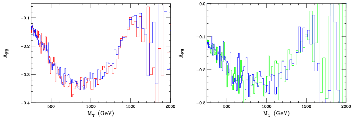
Figure 7: The y -integrated value of A_{FB} , as a function of the transverse mass, assuming a mass of 1.5 TeV for the W'^+(W'^-) in the left (right) panel. Here an integrated luminosity of 300 \text{ fb}^{-1} has been assumed. The two essentially indistinguishable histograms correspond to the two possible choices of the helicity, h_{W'} = \pm 1 .
